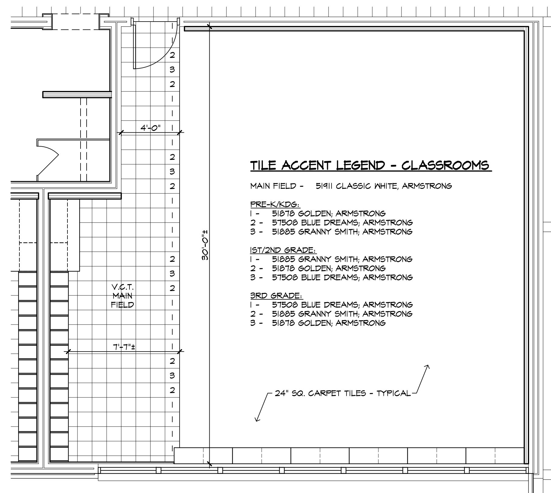
2 A2.5 RM. 147 TILE PATTERN 1/4" = 1'-0" RM. 135, 138, 141, 144, 146, 150 & 151 SIMILAR
