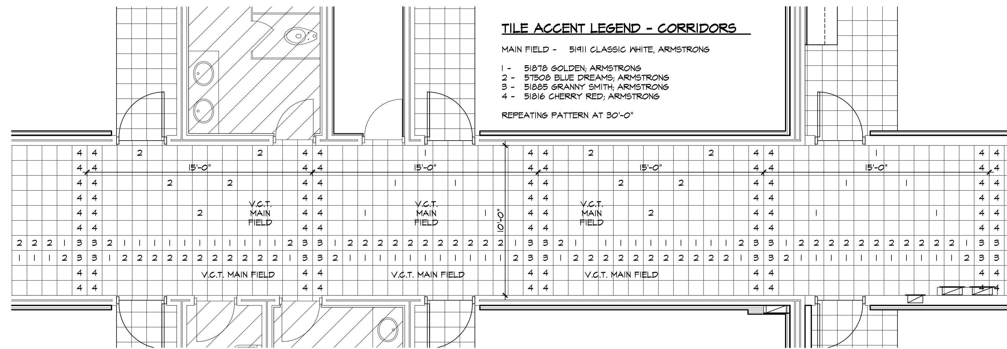
3 A2.5 TYPICAL CORRIDOR TILE PATTERN 1/4" = 1'-0"
