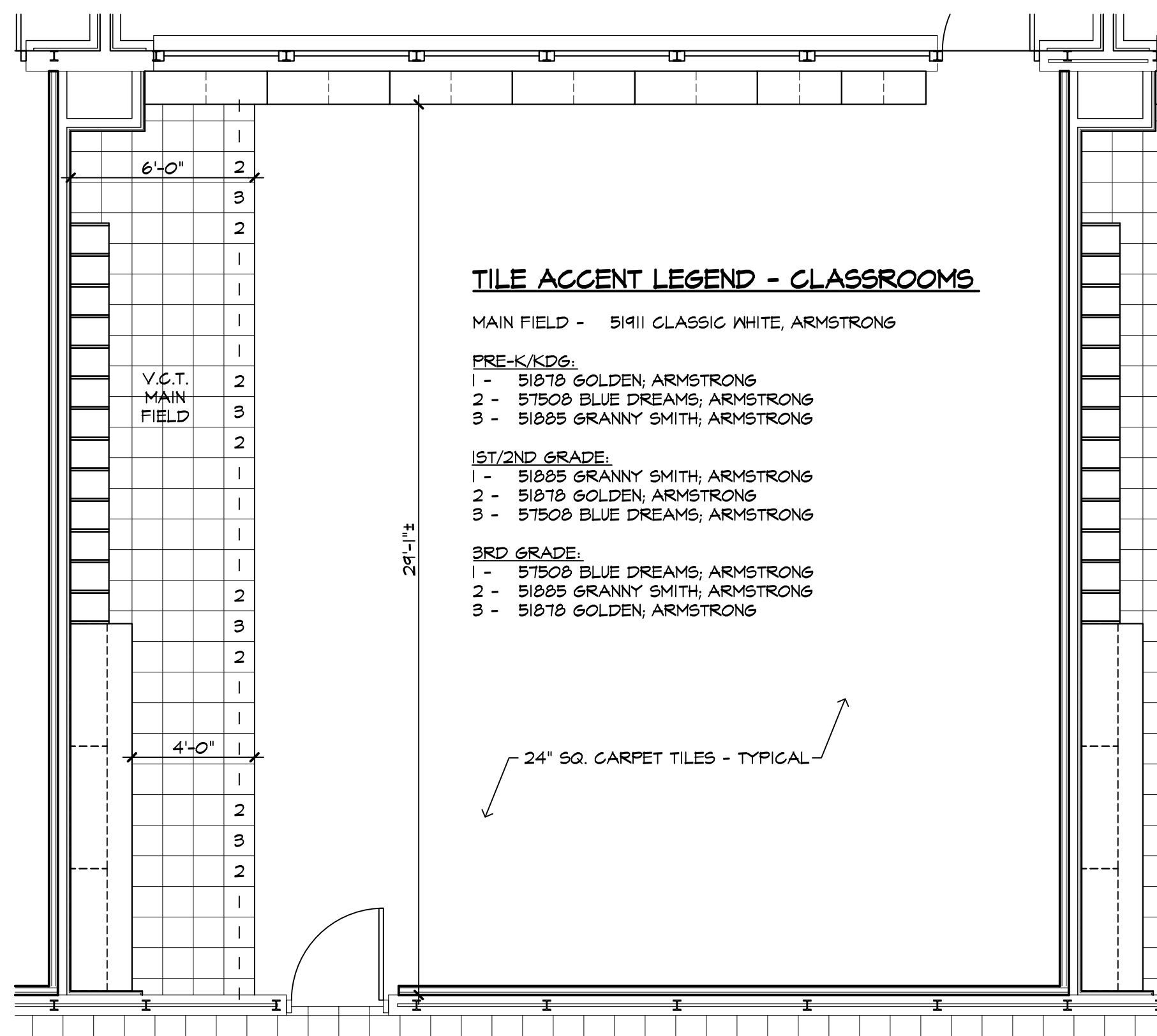
1 A2.5 RM. 104 TILE PATTERN 1/4" = 1'-0" RM. 102, 106, 110A, 112, 114, 133, 136, 128, 129, 131, 132 & 134 SIMILAR
